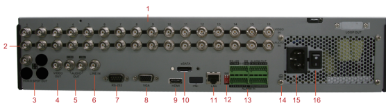
Rear Panel of DS-8116HDI-ST
